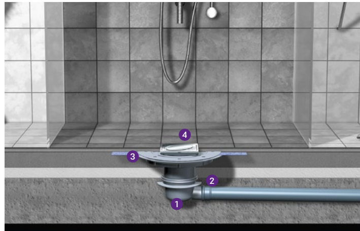
1 Drain 2 Outlet 3 Adhesive flange 4 Steel cover
